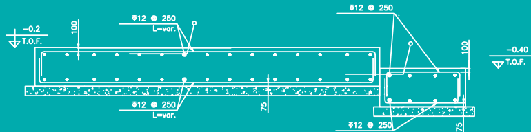
SECTION 5-5 SCALE: 1:20 REINFORCEMENT
